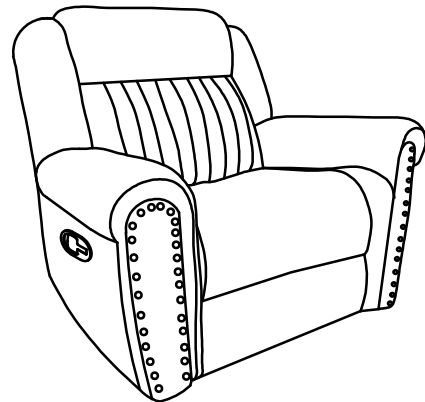
Step 4 # Completed
